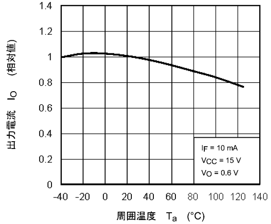
図 12.2.8 Normalized I_O - T_a
