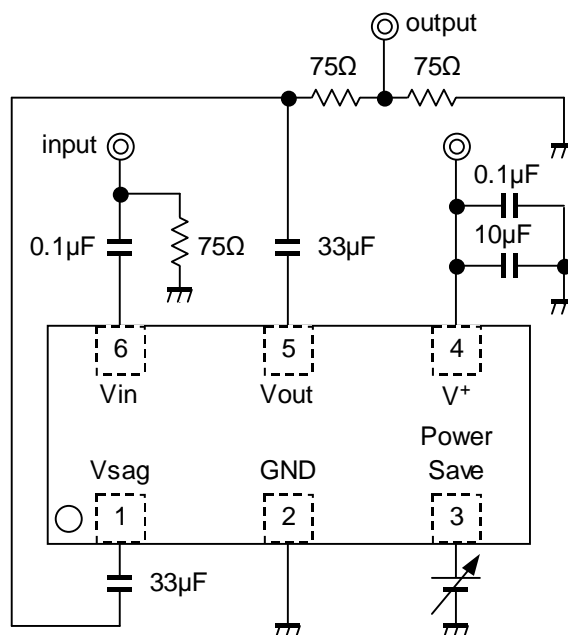
ESON6-G1 (Top View)
